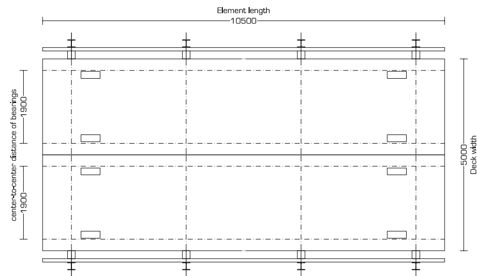
Top view JSB 200 series - 5,00m Deck width
