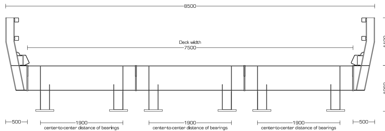
Cross view JSB 200 series - 1,06m Construction height
