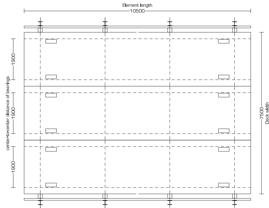
Top view JSB 200 series - 7,50m Deck width
