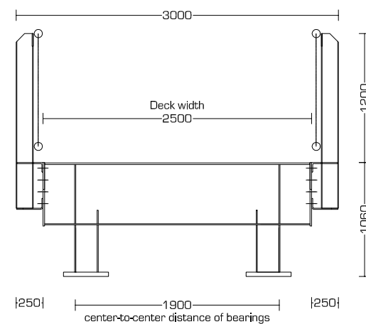
Cross view JSB 200 series - 1,06m Construction height
