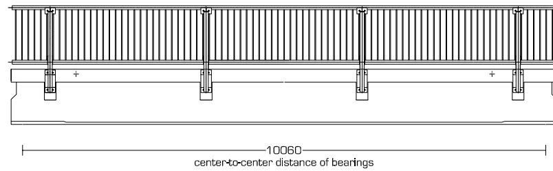
Side view JSB 200 series - 10,50m Free span
