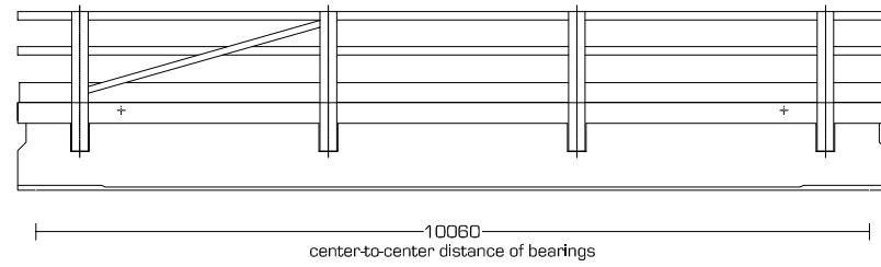
Side view JSB 200 series - 10,50m Free span
