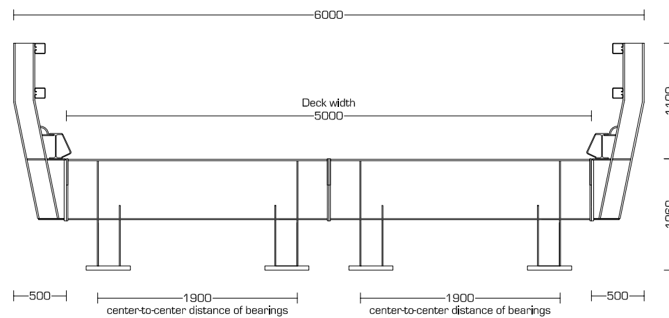
Cross view JSB 200 series - 1,06m Construction height
