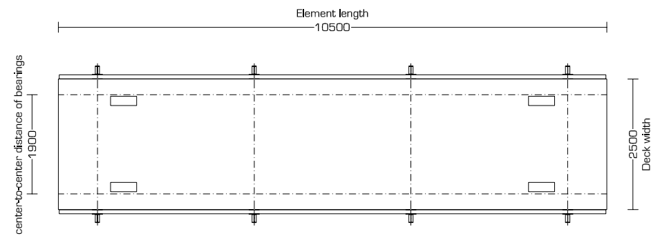
Top view JSB 200 series - 2,50m Deck width
