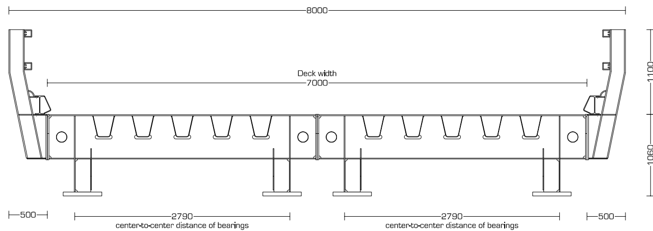
Cross view JSB 300 series - 1,06m Construction height [1-50]
