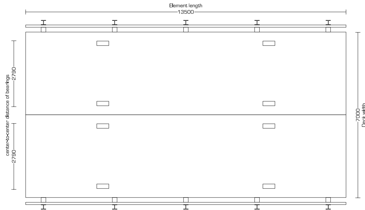
Top view JSB 300 series - 7,00m Deck width [1-100]
