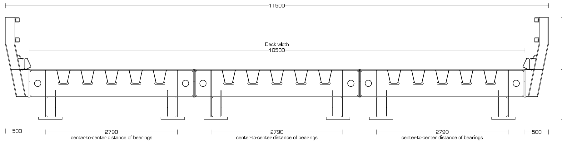
Cross view JSB 300 series - 1,06m Construction height [1-50]
