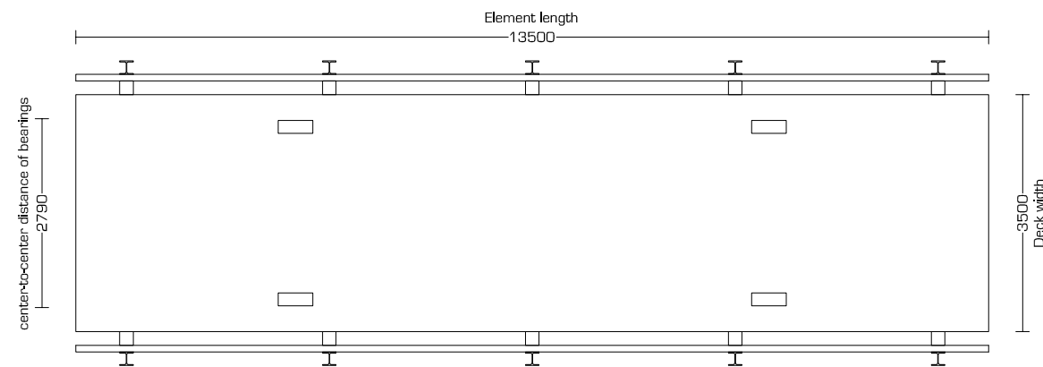
Top view JSB 300 series - 3,50m Deck width [1-100]
