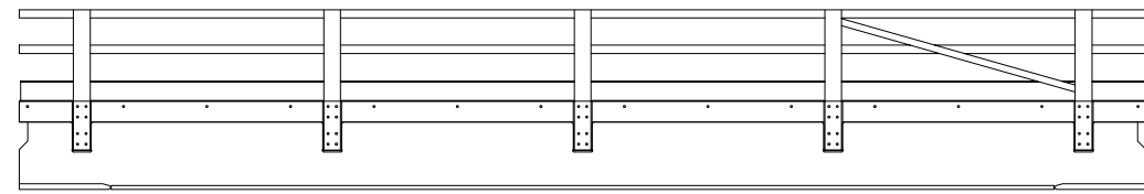
Side view JSB 300 series - 13,50m Free span [1-100]
