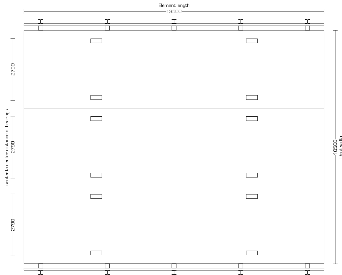
Top view JSB 300 series - 10,50m Deck width [1-100]
