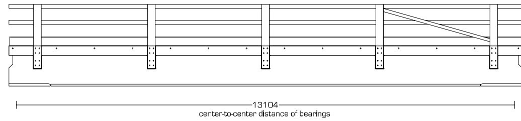
Side view JSB 300 series - 13,50m Free span [1-100]
