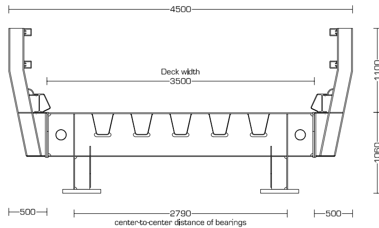
Cross view JSB 300 series - 1,06m Construction height [1-50]
